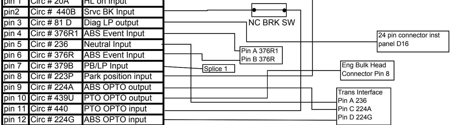
12 Pin Connector J2
